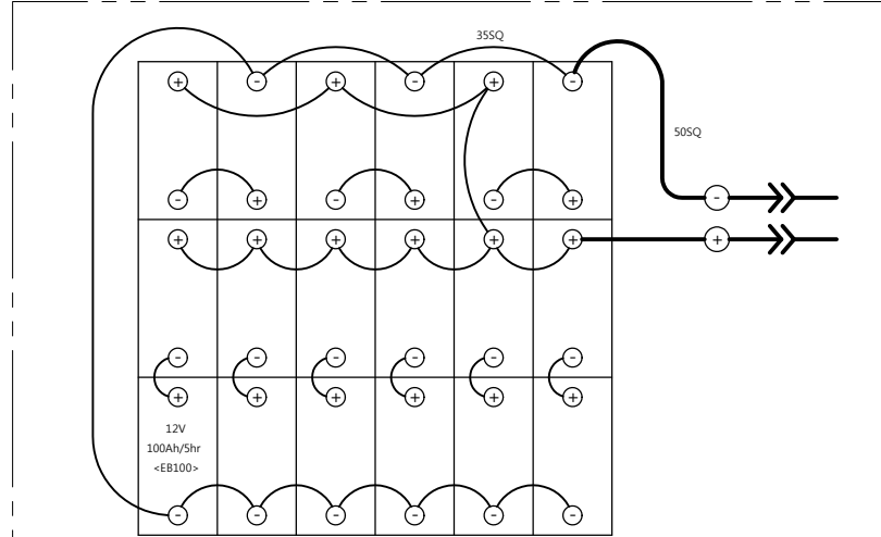
< BATTERY CONNECTION WIRING DIAGRAM 24Vx900Ah >
