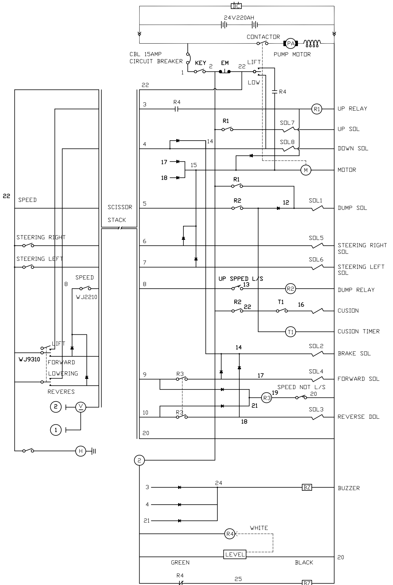
Figure 3-1, Electrical Schematic - Standard (SSL-1932)
